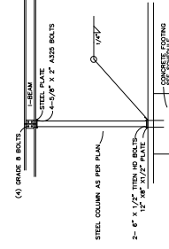
16 I-BEAM/COLUMN NTS
