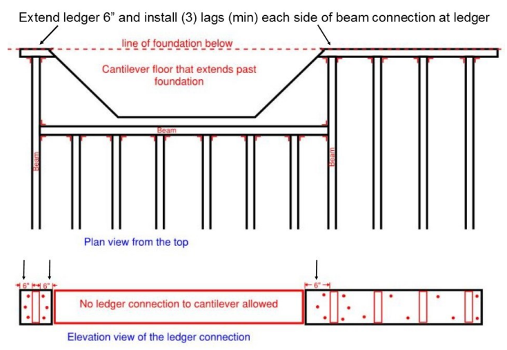
LEDGER DETAILS
