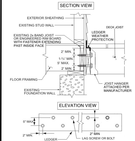
LEDGER DETAILS
