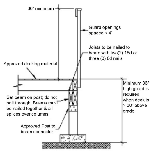
GUARD DETAILS
