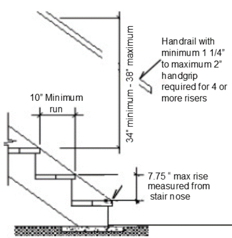
STAIR DETAILS
