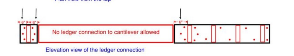
CANTILEVER DETAILS
