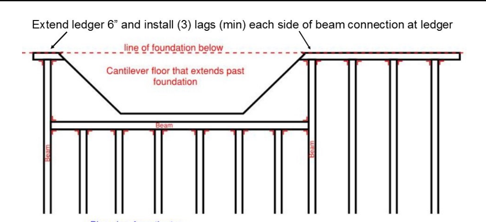
Plan view from the top
